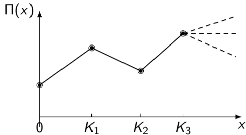
Figure 1: Illustration of a profit function \Pi(x) on x > 0 with finitely many affine branches and grid nodes (kinks) at S = \{0, K_1, K_2, K_3\} . Since \Pi is affine between consecutive nodes, its minimum over (0, \infty) is attained by checking the node values, including the boundary point x = 0 , provided the tail slope condition prevents \Pi(x) \rightarrow -\infty as x \rightarrow \infty . The three dashed rays depict alternative tail slopes on the last branch: increasing, flat, and decreasing.
